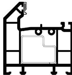
72MM PVC-U THRESHOLD (BEVELLED)
