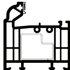
72MM PVC-U THRESHOLD (OVOLO)
